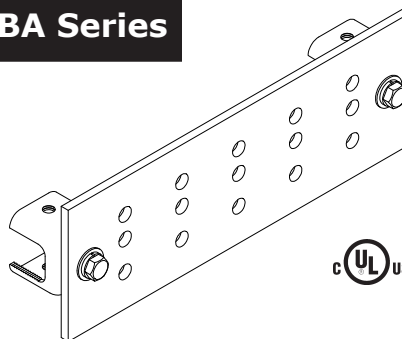
G round B ar with Stainless Steel Angle A dapters
