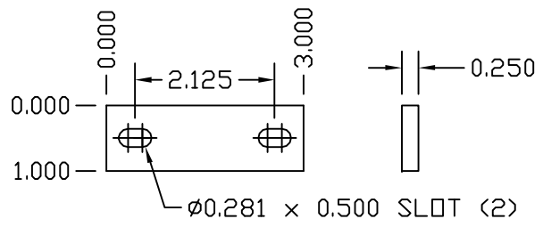
TINNED COPPER SPLICE PLATE
