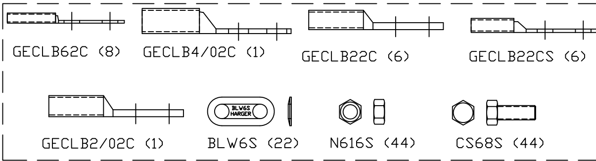
HARDWARE KIT
