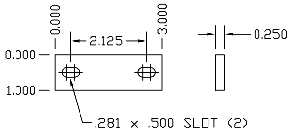
SPLICE PLATE
