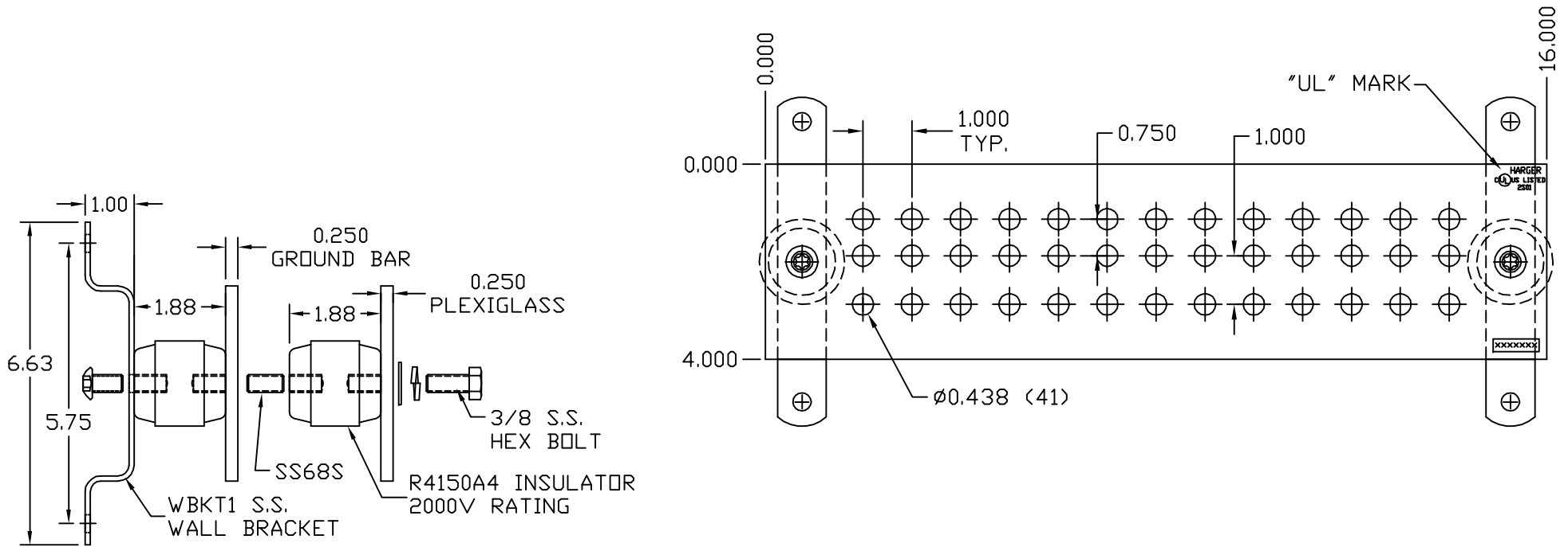
COPPER GROUND BAR ASSEMBLY
