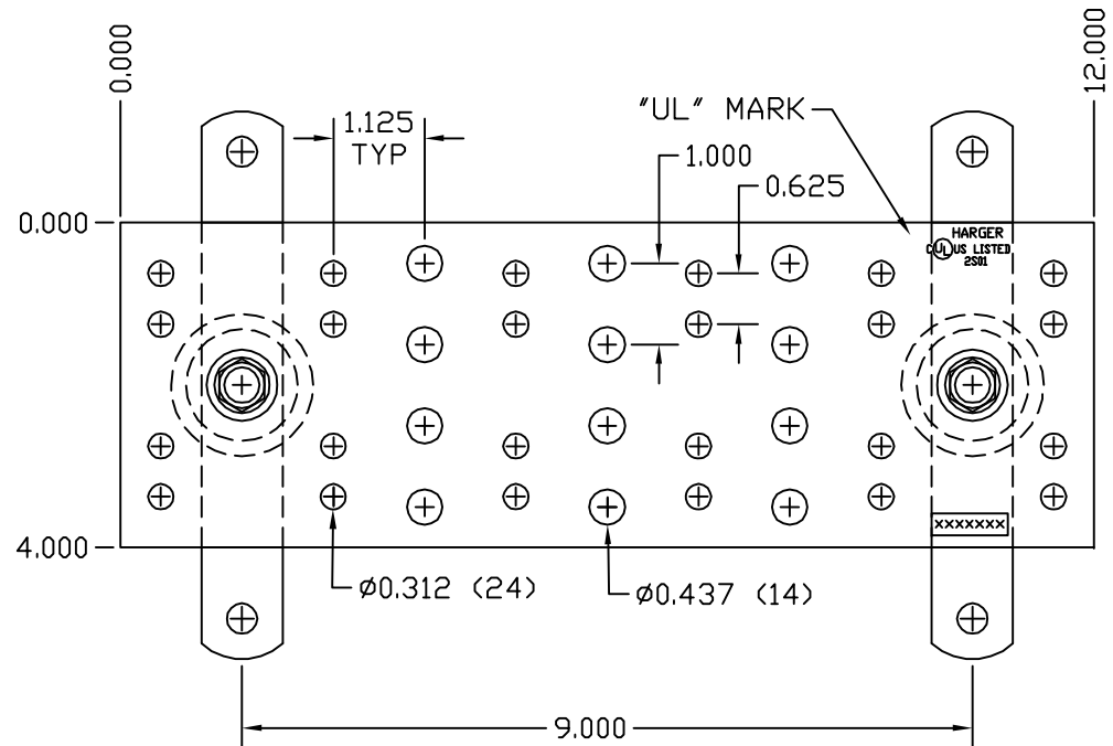
COPPER GROUND BAR ASSEMBLY
