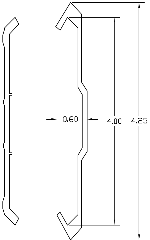
CROSS SECTION
