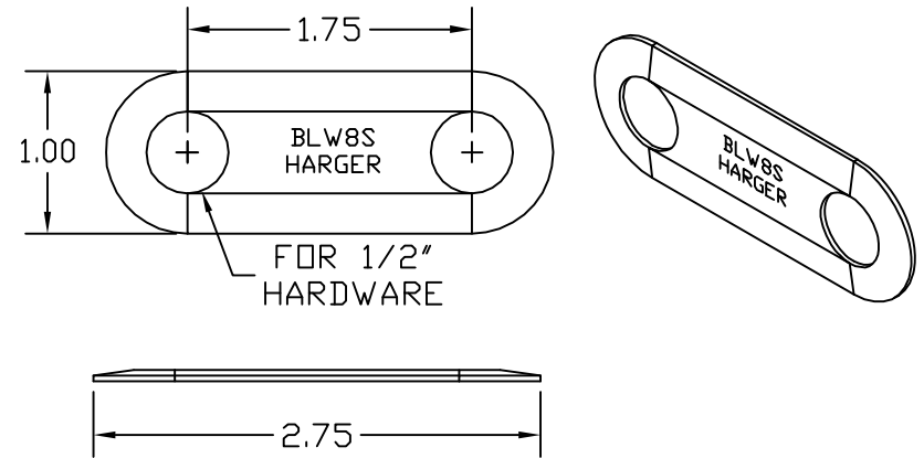
STAINLESS STEEL CUPPED WASHER
