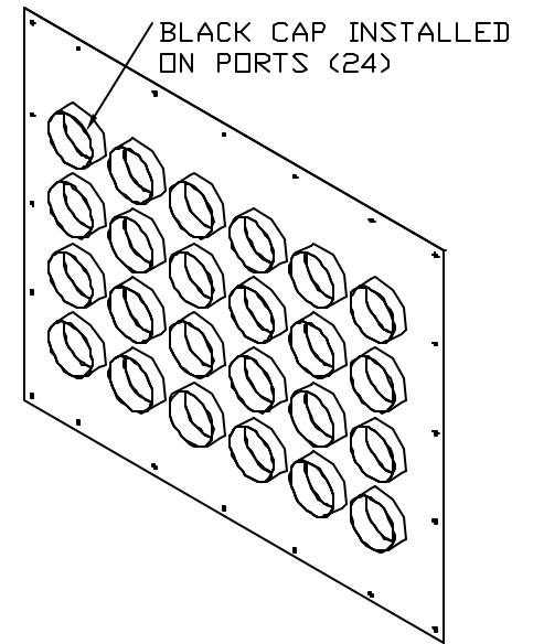
24 UNIT ENTRANCE PANEL 4X6 MAPLE POWDERCOAT FINISH
