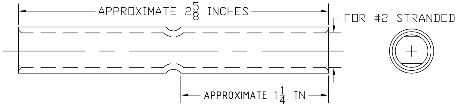
2 AWG STR. (∅0.292) LONG BARREL BUTT SPLICE
