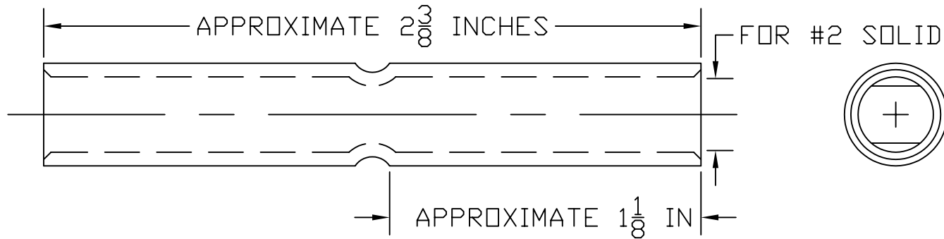
2 AWG SOLID (∅0.260) LONG BARREL BUTT SPLICE
