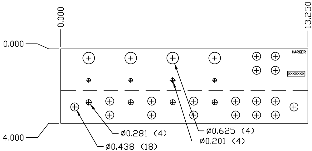
FLAT BAR LAYOUT
