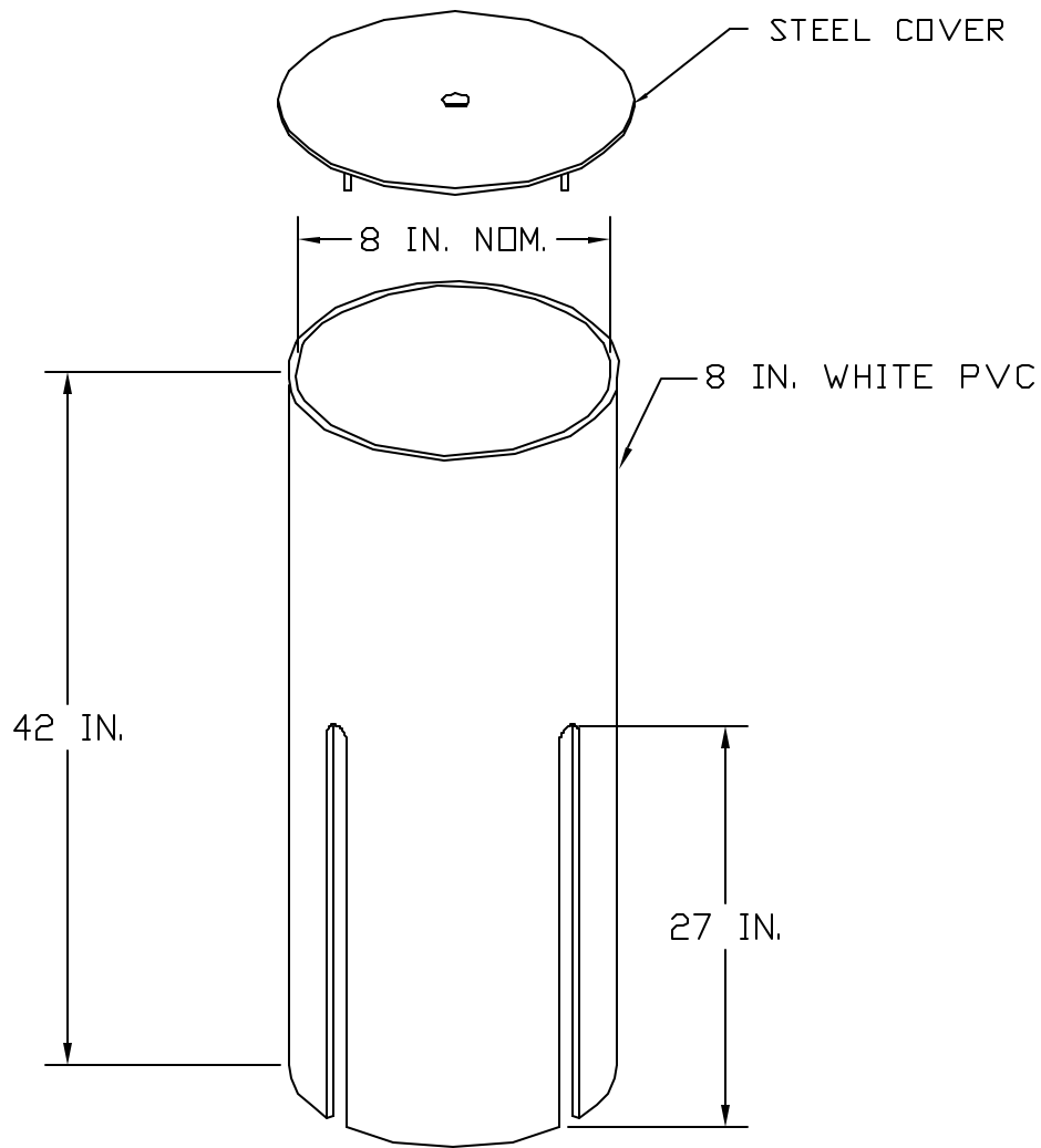
GROUND TEST WELL
