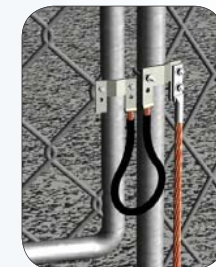
6. Flexible Gate Jumper
