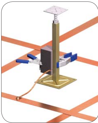
MH4 required for mounting all VHO molds to the raised floor pedestal during welding.
