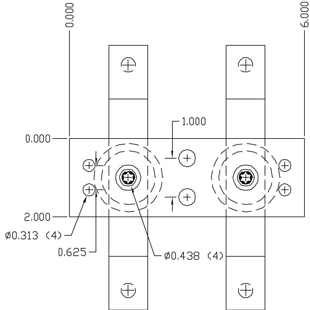
GROUND BAR ASSEMBLY
