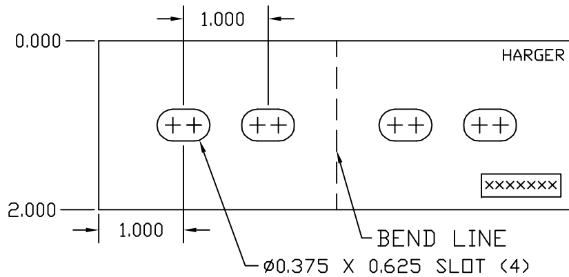
FLAT LAYOUT
