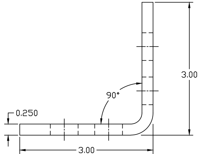
COPPER GROUND BUSBAR 90° ELBOW
