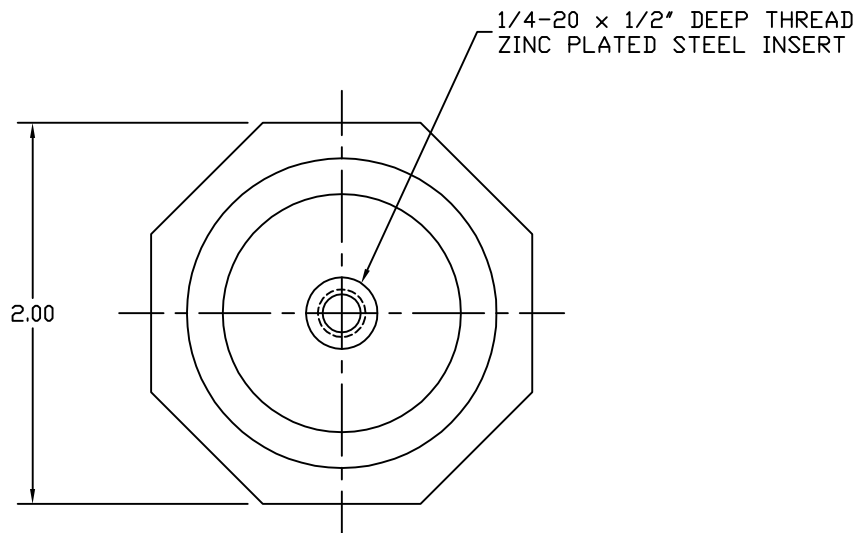
STANDOFF INSULATOR
