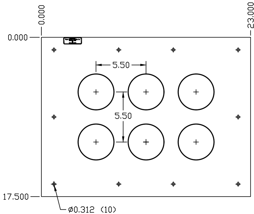
ALUMINUM ENTRY PANEL
